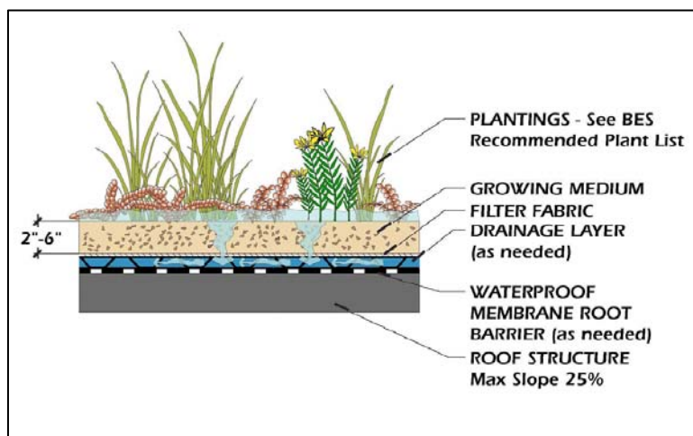
Figure 7.27: Extensive Green Roof System
