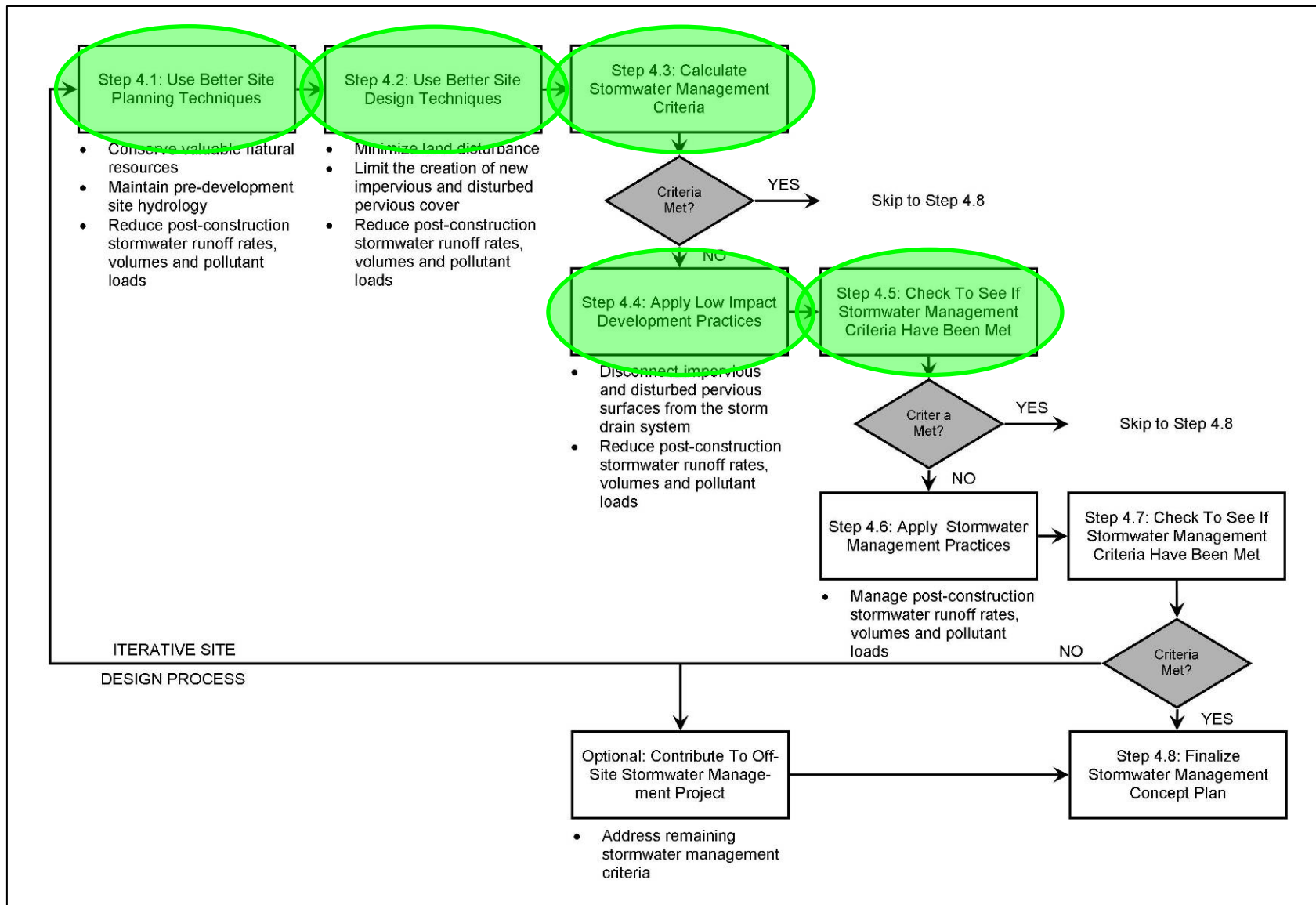
Figure 7.4: Using Green Infrastructure Practices During the Creation of a Stormwater Management Concept Plan
