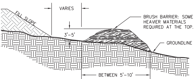
Figure 1. Brush Barrier (Sd1-BB)
